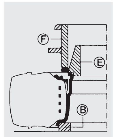
Inserting locking ring
