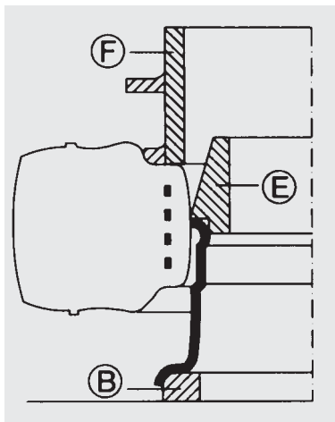
Pressing a tyre on
