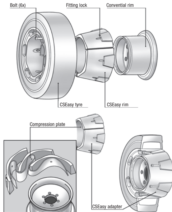
The inner adapter consists of three segments and a rubber layer (compression plate) which are pre-fitted.
